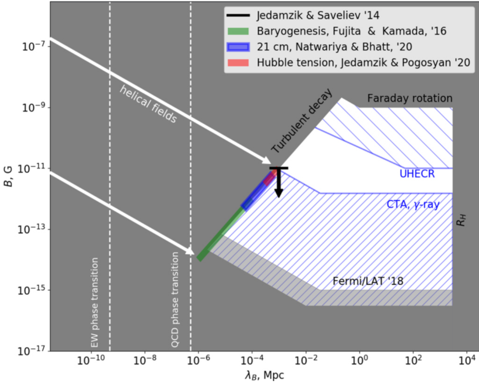
Figure 1. from Sensitivity Reach of Gamma-Ray Measurements for Strong Cosmological Magnetic Fields null 2021 APJ 906 116 doi:10.3847/1538-4357/abc697 https://dx.doi.org/10.3847/1538-4357/abc697 © 2021. The American Astronomical Society. All rights reserved.
