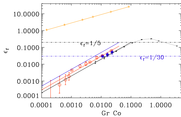
Figure 1: One (unknown) point on the orange line corresponds to Run A2. The line is relatively low, so mean-field dynamo action is only possible for large values of \epsilon_f or large eddies. poum_0dep_g08
