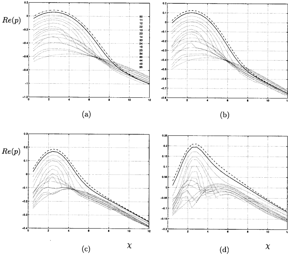
FIGURE 3 Growth rates Re(p) versus \chi , for k = 1/5 and (a) R_m = 0.75 , (b) R_m = 1 , (c) R_m = 2 and (d) R_m = 4 . The dashed curves correspond to the solutions with a = b = 0 , the solid curves to those with a = b = 1 and N = 10 , and the dotted curves to the other solutions with finite length scales with a/N and b/N as given for N = 10 in Table I. The labels ab on the right of (a) belong in this order to the left ends of the curves. In (b), (c) and (d) the first eight of these labels have to be assigned to the eight upper left ends of the curves.
