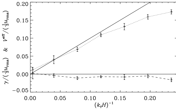
FIGURE 1. Dependence of V^{\text{eff}} (dotted line) and \gamma (dashed line) (here in the z direction) as a function of the inverse scale height H , normalized by the wavenumber k_f of the energy-carrying eddies. The turbulent pumping velocity \gamma caused by the non-uniformity of the turbulent r.m.s. velocity (solid line) in a non-stratified turbulence. Here the symbol H is used either for the density scale height, H = \lambda^{-1} , or for the characteristic scale of the non-uniformity of the turbulent r.m.s. velocity, H^{-1} = \nabla u_{\text{rms}}/u_{\text{rms}} .
